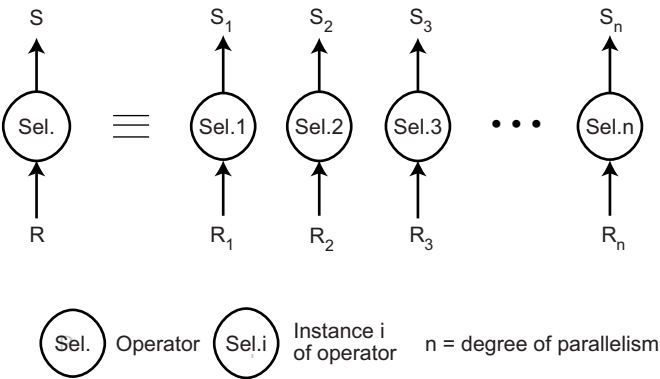
Fig. 14.11 Intra-operator Parallelism
